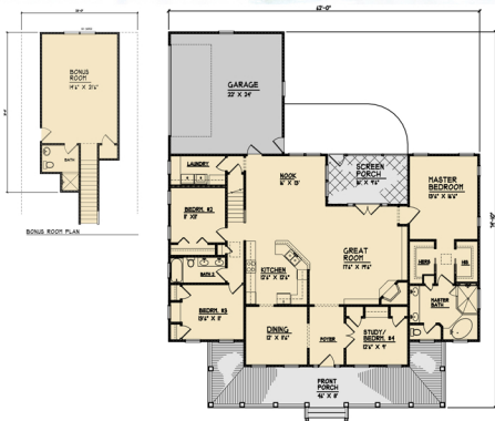
FLOOR PLAN
