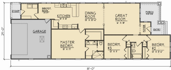
FLOOR PLAN
